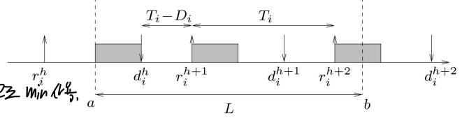
Fig. 2. Densest possible packing of jobs of task \tau_i in interval [a, b] .
